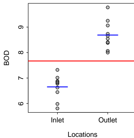
Figure 1.1. Biological oxygen demand (BOD) measurements at two locations – an inlet and an outlet. The red horizontal line represents the simple model of a grand mean for both groups. The two blue horizontal lines represent the full model of separate means for each group.
